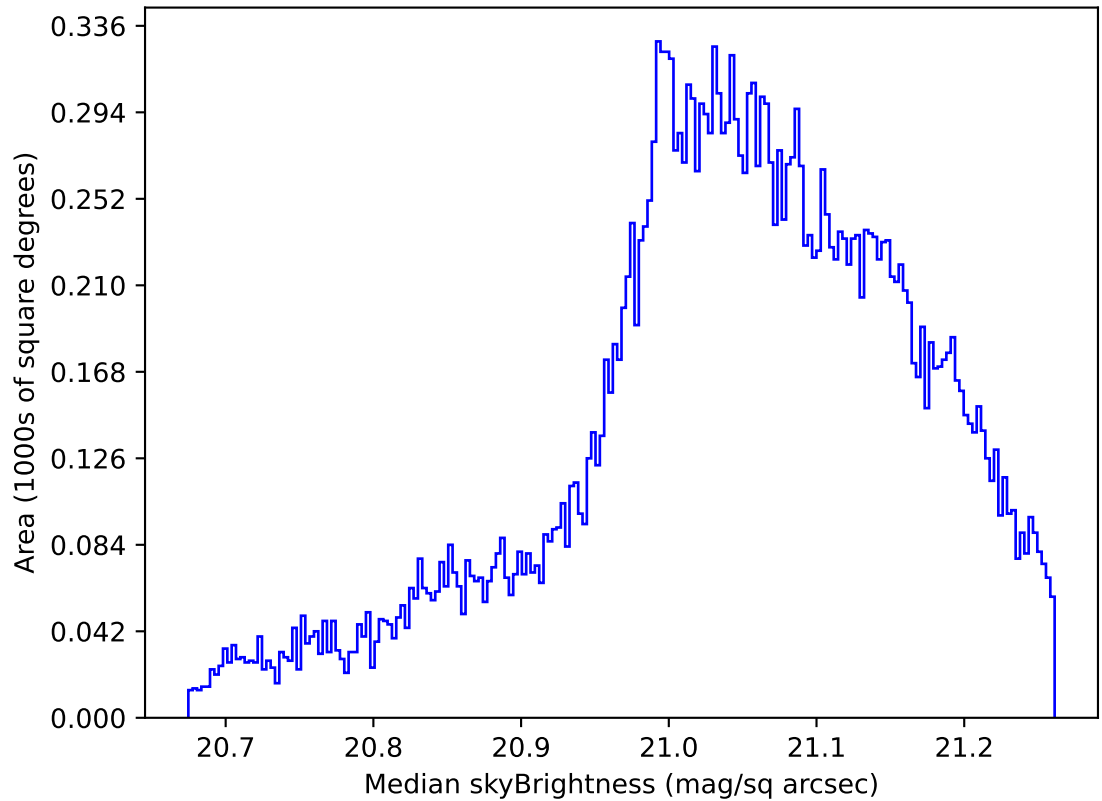
too_elab_heavy_r128_d3_gz_v3.4_10yrs All sky r band: Median skyBrightness
