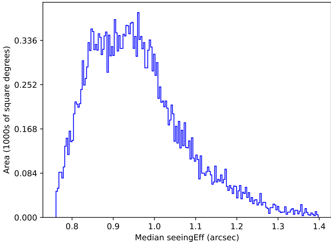
too_elab_heavy_r128_d3_gz_v3.4_10yrs Yr 1 z band: Median seeingEff
