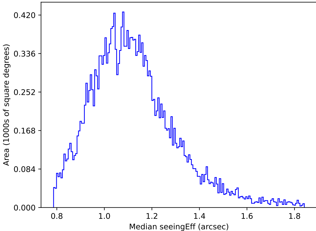
too_elab_heavy_r128_d3_gz_v3.4_10yrs Yr 1 u band: Median seeingEff
