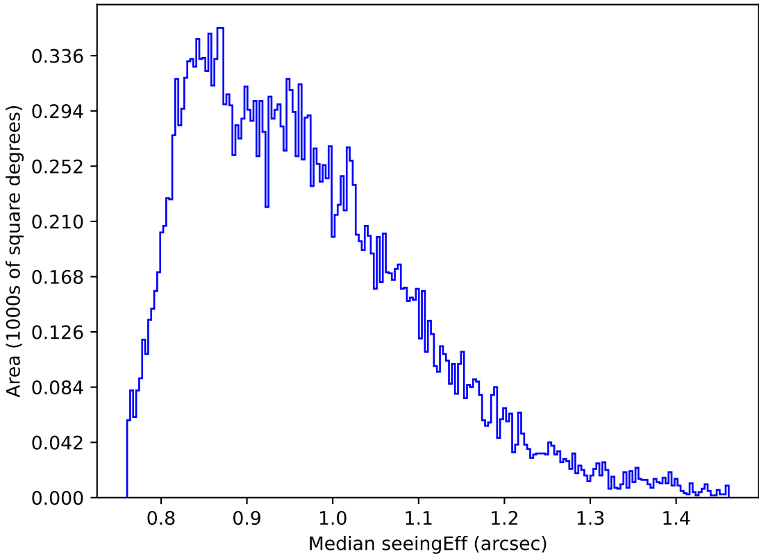
too_elab_heavy_r128_d3_gz_v3.4_10yrs Yr 1 i band: Median seeingEff
