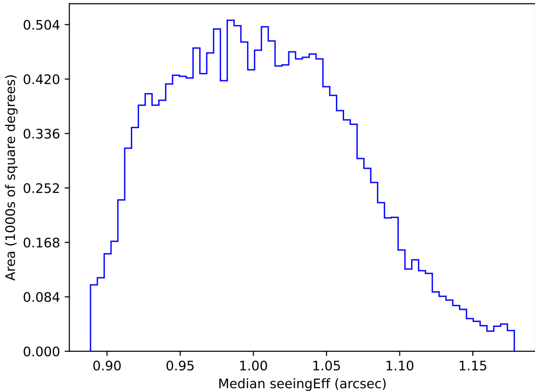
too_elab_heavy_r128_d3_gz_v3.4_10yrs WFD y band: Median seeingEff
