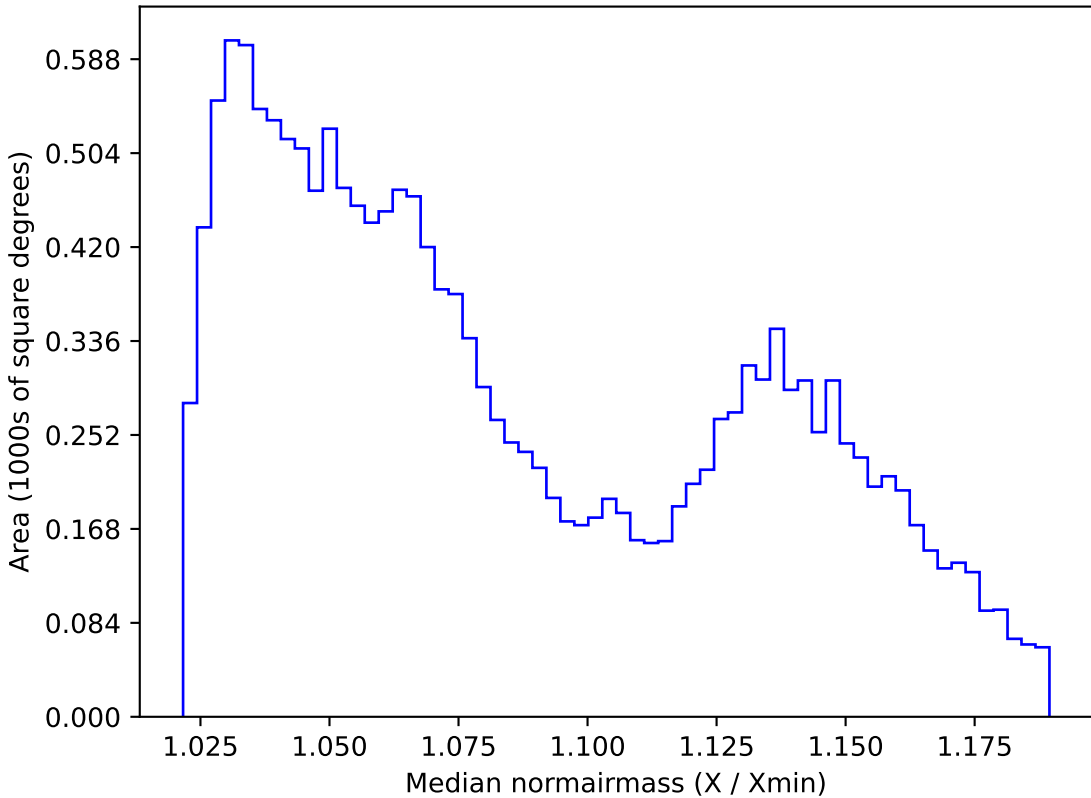
too_elab_heavy_r128_d3_gz_v3.4_10yrs WFD i band: Median normairmass
