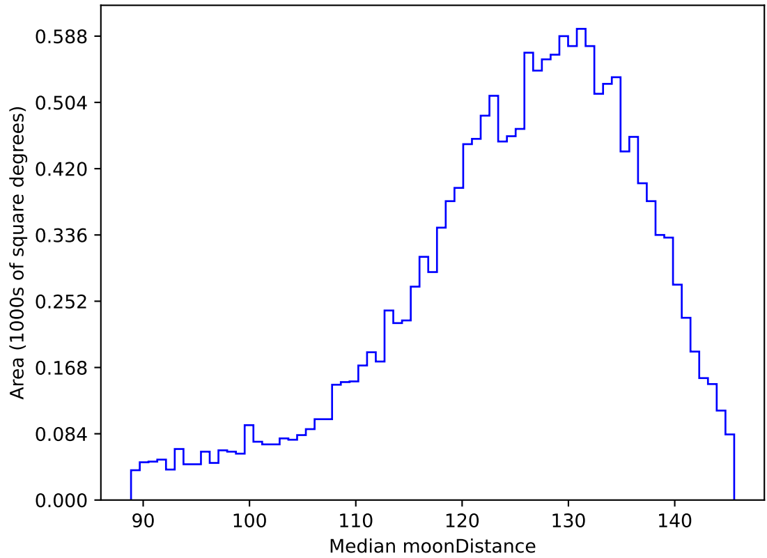
too_elab_heavy_r128_d3_gz_v3.4_10yrs WFD u band: Median moonDistance
