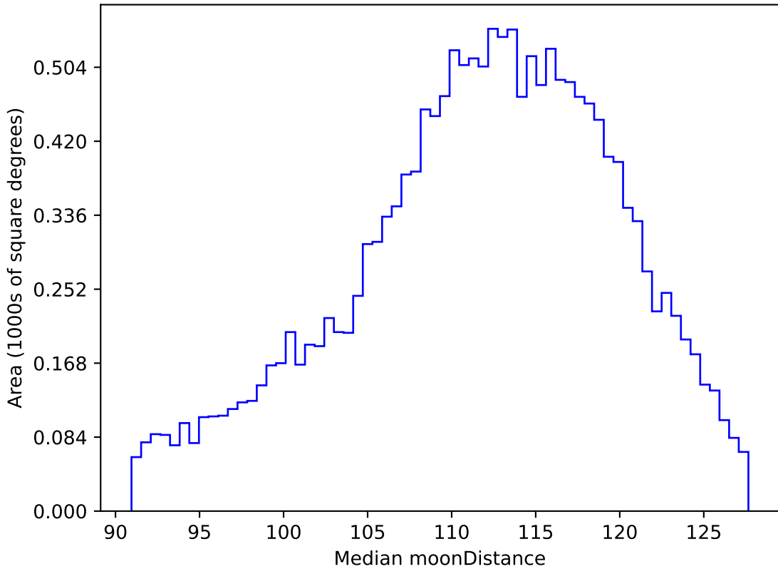
too_elab_heavy_r128_d3_gz_v3.4_10yrs WFD r band: Median moonDistance
