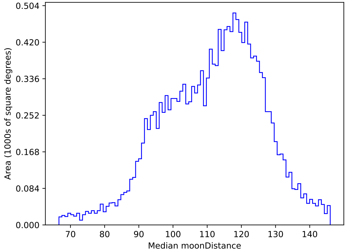
too_elab_heavy_r128_d3_gz_v3.4_10yrs WFD g band: Median moonDistance
