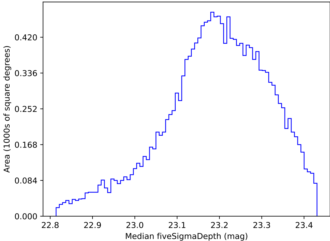
too_elab_heavy_r128_d3_gz_v3.4_10yrs WFD u band: Median fiveSigmaDepth
