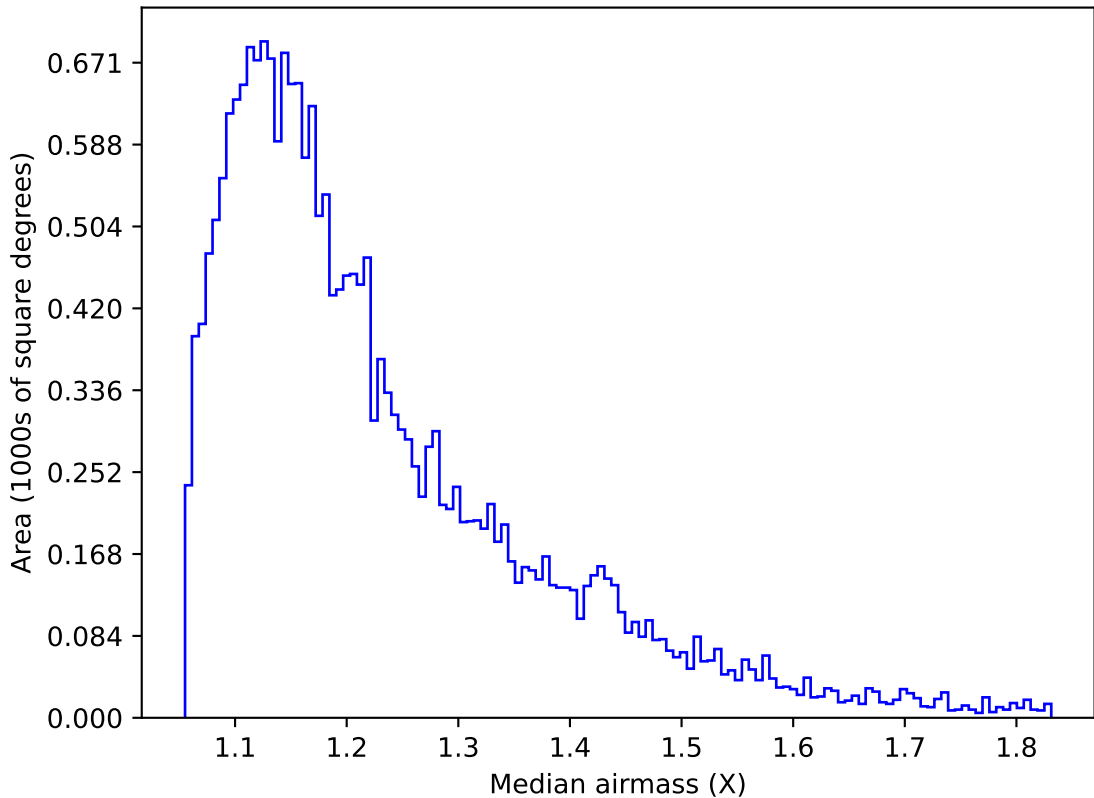
too_elab_heavy_r128_d3_gz_v3.4_10yrs Yr 1 u band: Median airmass
