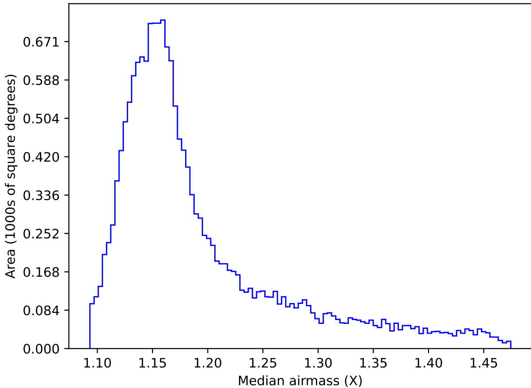
too_elab_heavy_r128_d3_gz_v3.4_10yrs WFD z band: Median airmass
