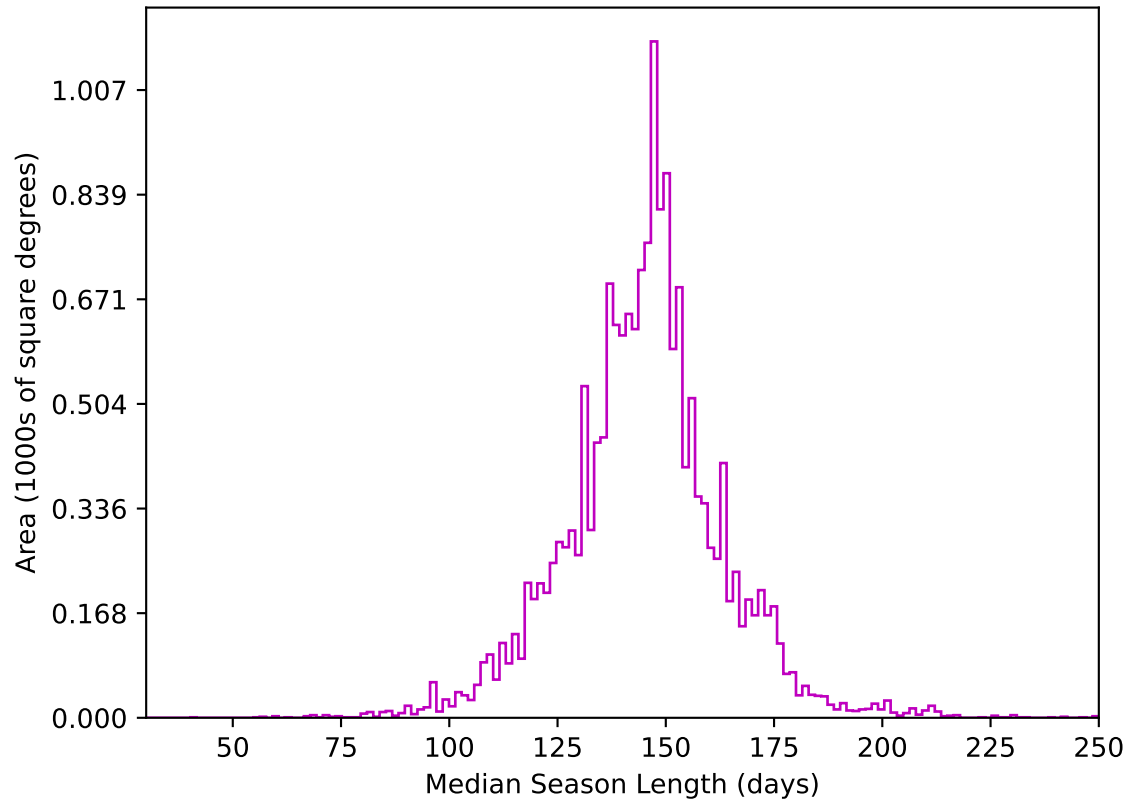
too_elab_heavy_r128_d3_gz_v3.4_10yrs WFD z band: Median Season Length
