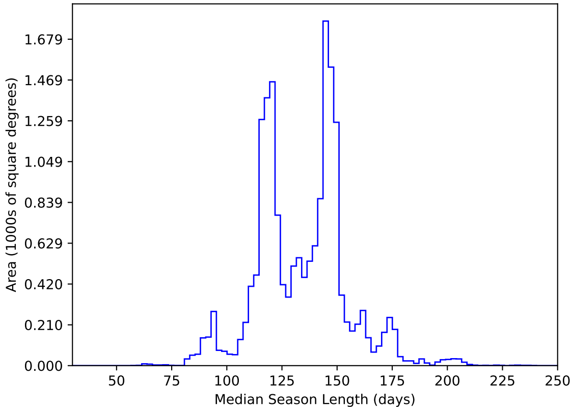
too_elab_heavy_r128_d3_gz_v3.4_10yrs WFD y band: Median Season Length
