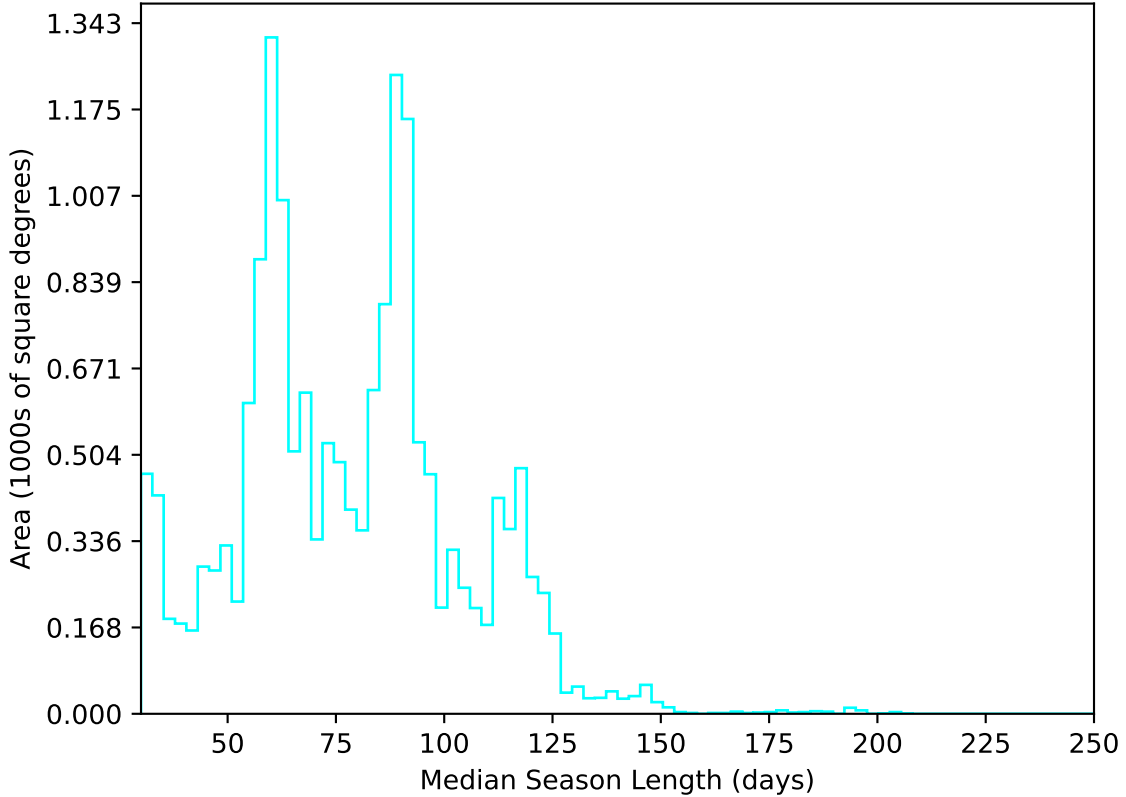
too_elab_heavy_r128_d3_gz_v3.4_10yrs WFD u band: Median Season Length
