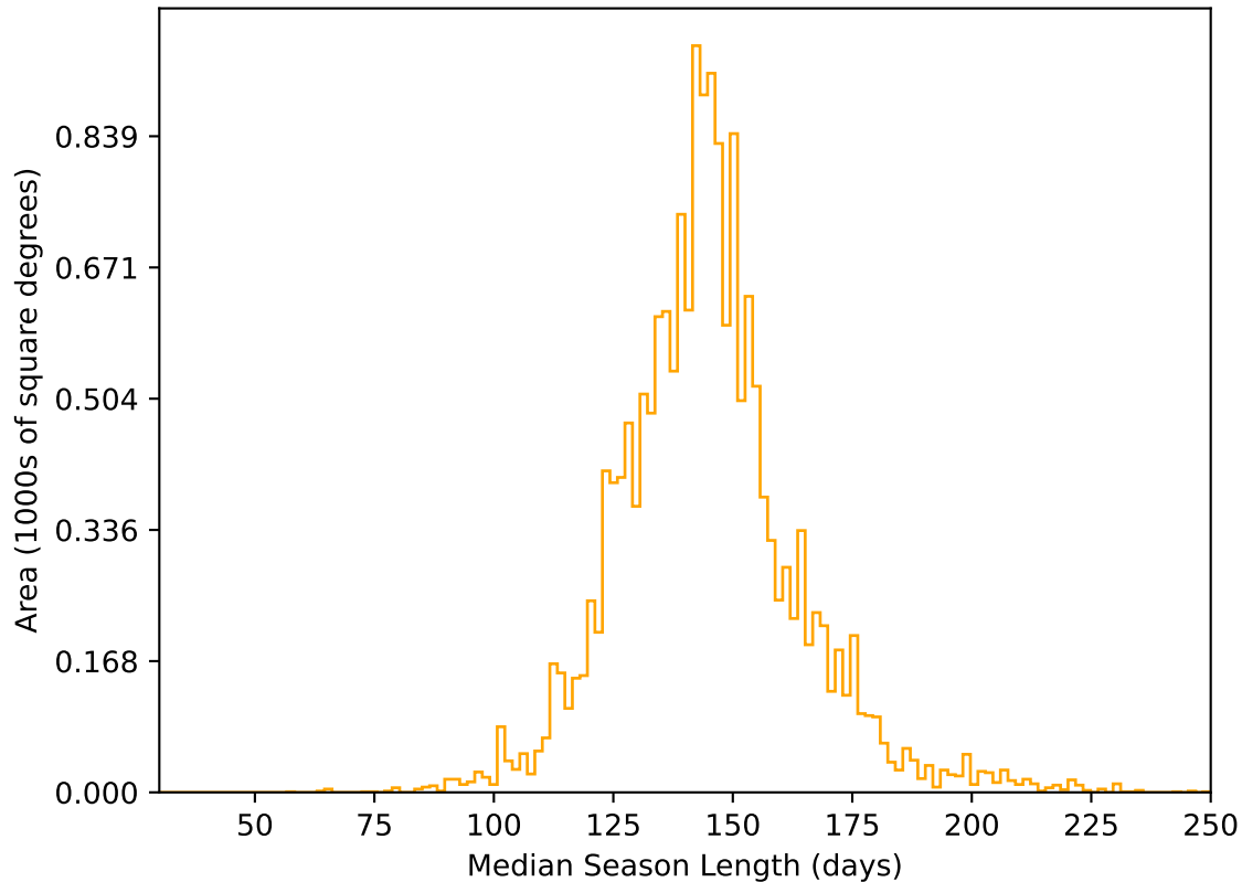
too_elab_heavy_r128_d3_gz_v3.4_10yrs WFD r band: Median Season Length
