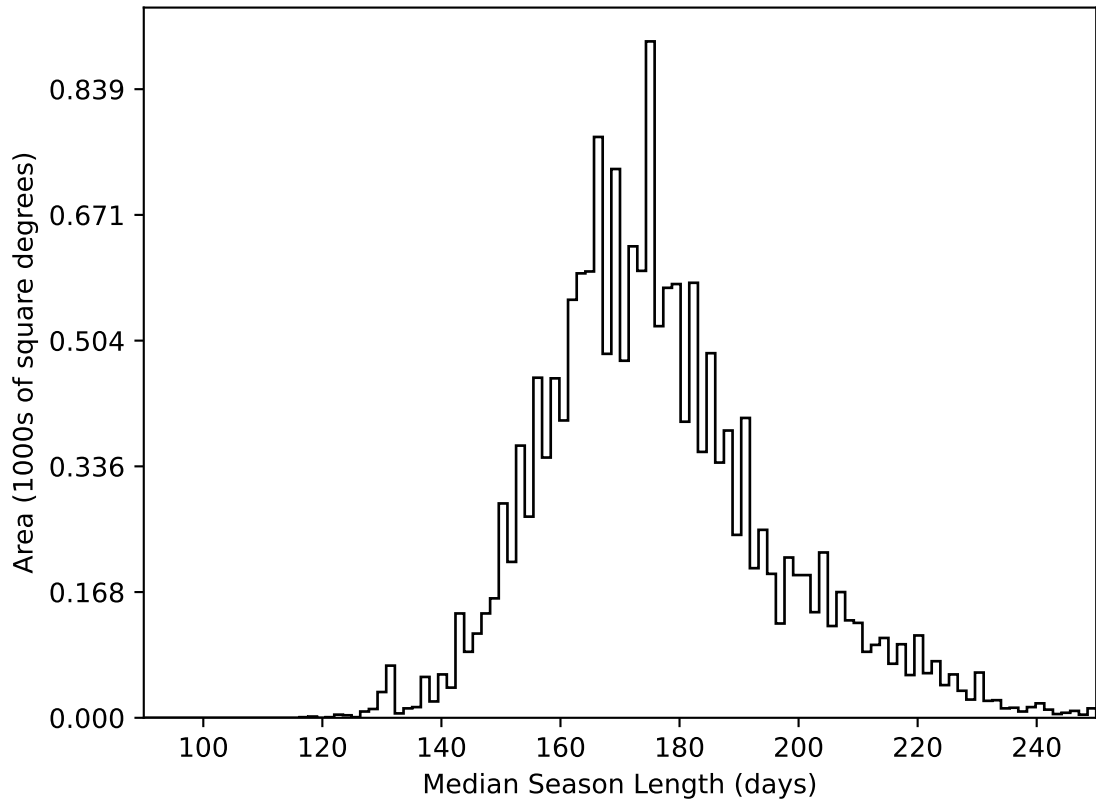
too_elab_heavy_r128_d3_gz_v3.4_10yrs WFD all bands: Median Season Length
