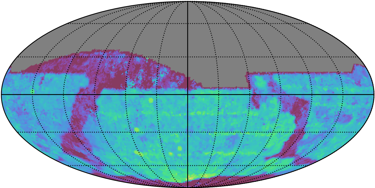
too_elab_heavy_r128_d3_gz_v3.4_10yrs All sky z band: Median Season Length
