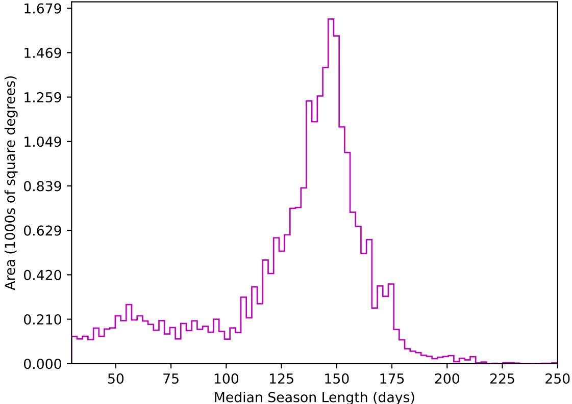
too_elab_heavy_r128_d3_gz_v3.4_10yrs All sky z band: Median Season Length
