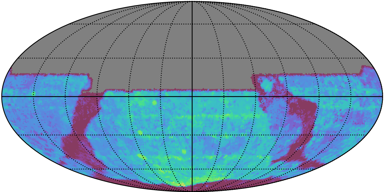
too_elab_heavy_r128_d3_gz_v3.4_10yrs All sky y band: Median Season Length
