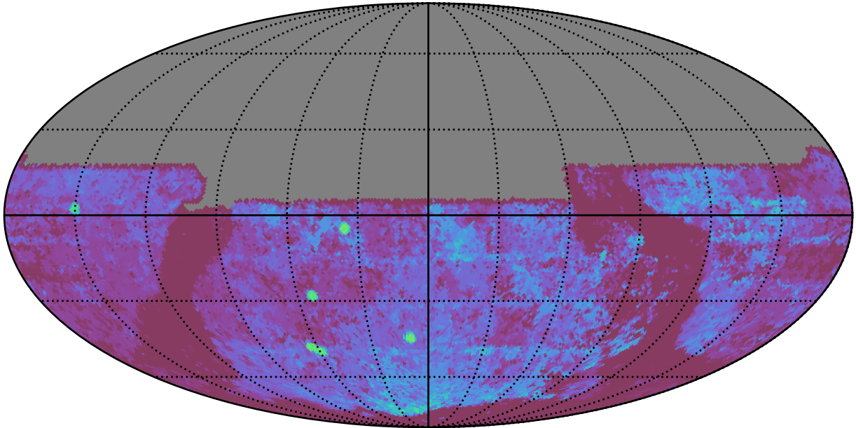
too_elab_heavy_r128_d3_gz_v3.4_10yrs All sky u band: Median Season Length
