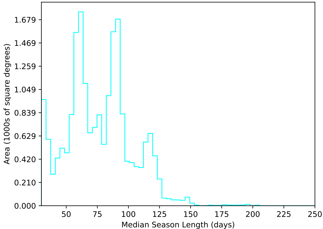
too_elab_heavy_r128_d3_gz_v3.4_10yrs All sky u band: Median Season Length
