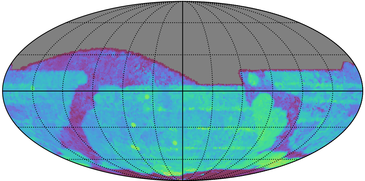
too_elab_heavy_r128_d3_gz_v3.4_10yrs All sky r band: Median Season Length
