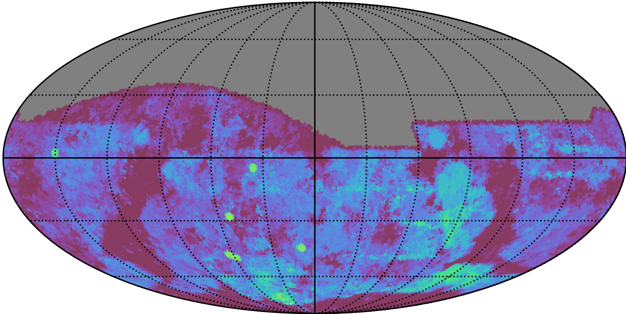
too_elab_heavy_r128_d3_gz_v3.4_10yrs All sky g band: Median Season Length
