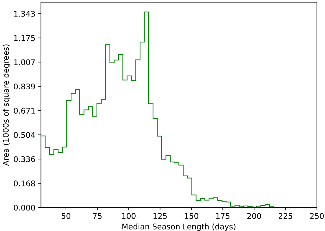
too_elab_heavy_r128_d3_gz_v3.4_10yrs All sky g band: Median Season Length
