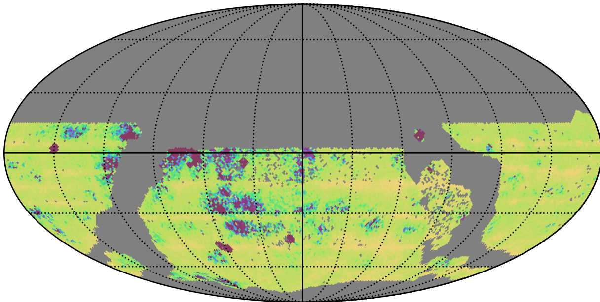
too_elab_heavy_r128_d3_gz_v3.4_10yrs WFD: Median Intra-Night Gap
