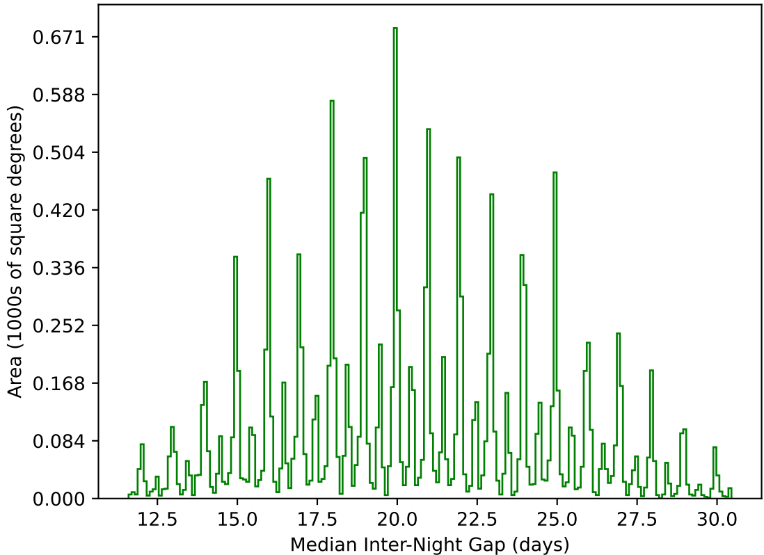
too_elab_heavy_r128_d3_gz_v3.4_10yrs WFD g band: Median Inter-Night Gap
