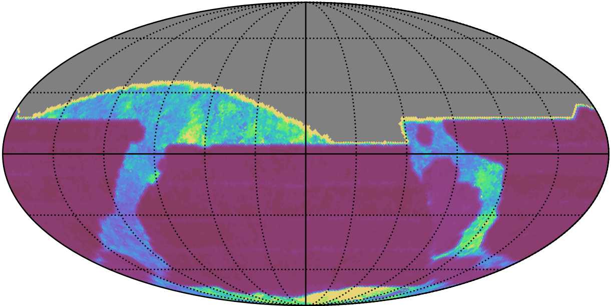
too_elab_heavy_r128_d3_gz_v3.4_10yrs All sky all bands: Median Inter-Night Gap
