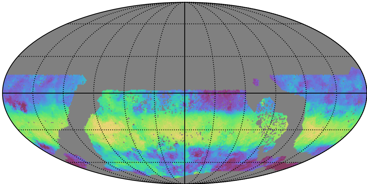
too_elab_heavy_r128_d3_gz_v3.4_10yrs WFD z band: Median HA
