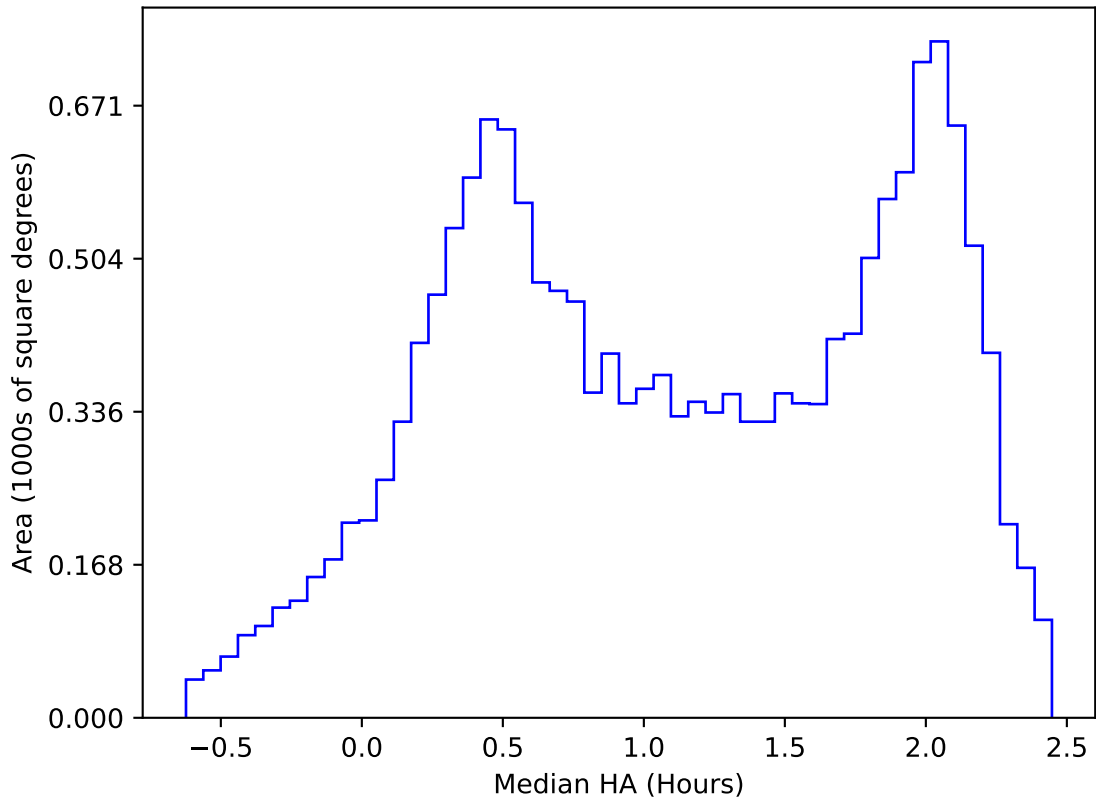
too_elab_heavy_r128_d3_gz_v3.4_10yrs WFD z band: Median HA
