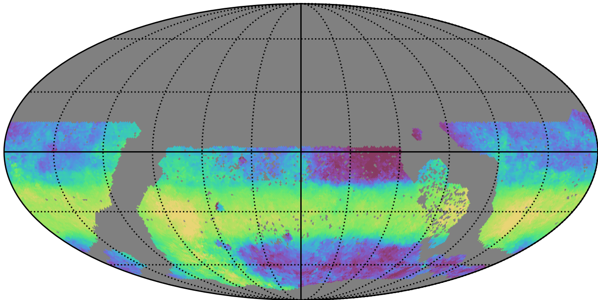
too_elab_heavy_r128_d3_gz_v3.4_10yrs WFD y band: Median HA
