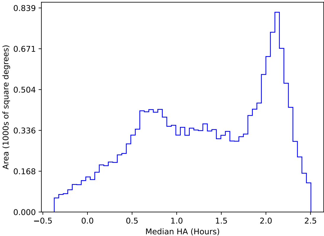
too_elab_heavy_r128_d3_gz_v3.4_10yrs WFD y band: Median HA
