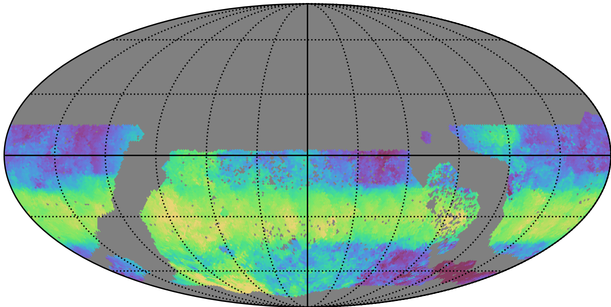
too_elab_heavy_r128_d3_gz_v3.4_10yrs WFD u band: Median HA
