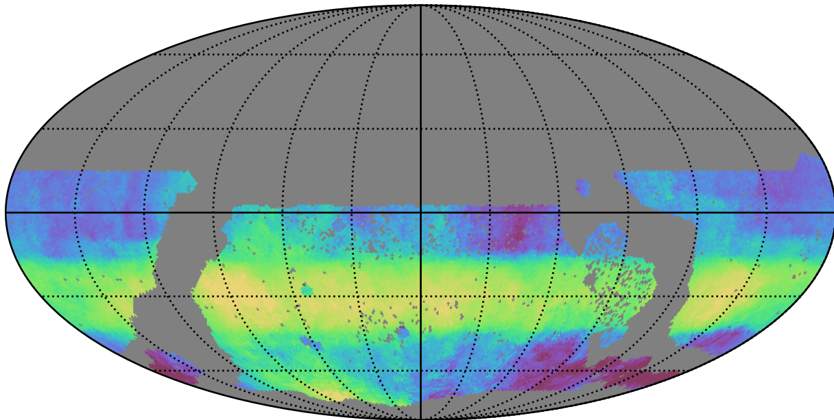
too_elab_heavy_r128_d3_gz_v3.4_10yrs WFD r band: Median HA
