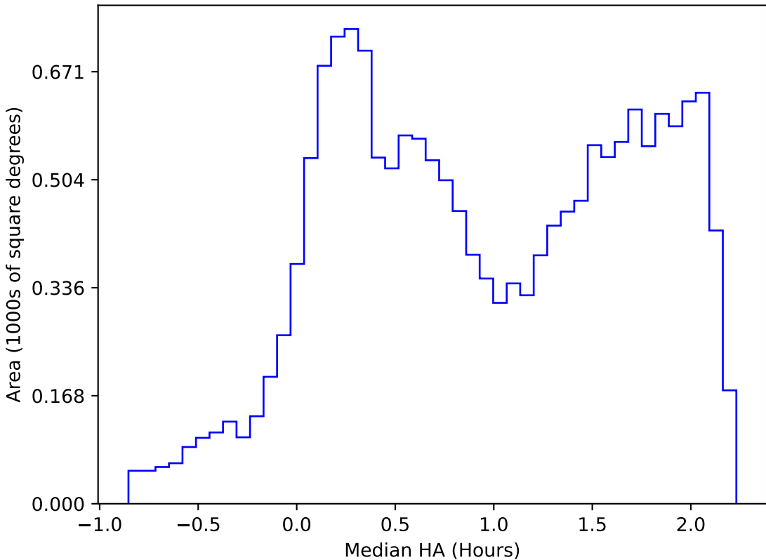
too_elab_heavy_r128_d3_gz_v3.4_10yrs WFD r band: Median HA
