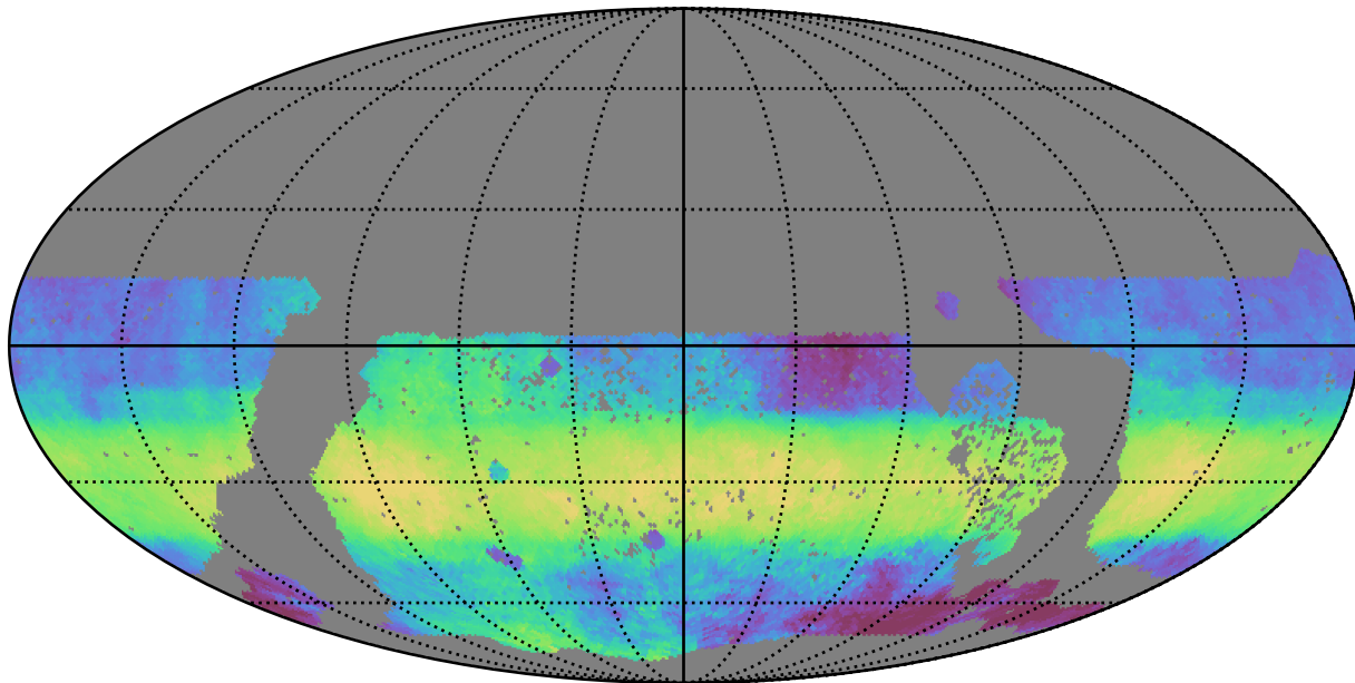
too_elab_heavy_r128_d3_gz_v3.4_10yrs WFD i band: Median HA
