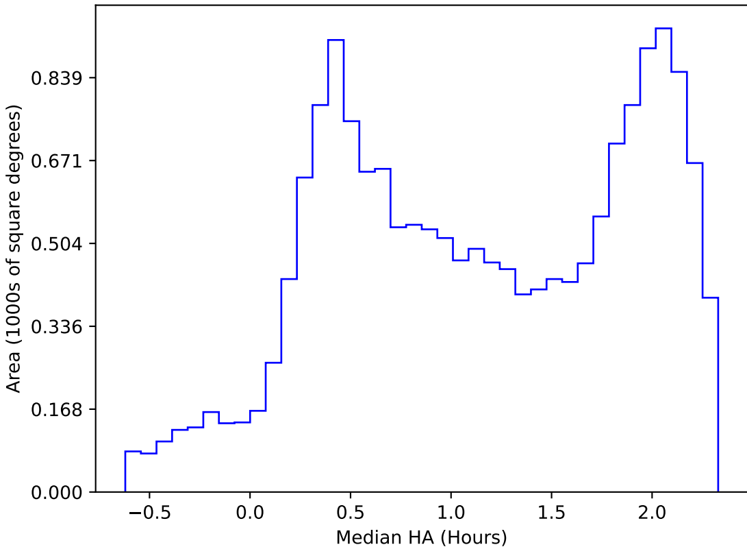
too_elab_heavy_r128_d3_gz_v3.4_10yrs WFD i band: Median HA
