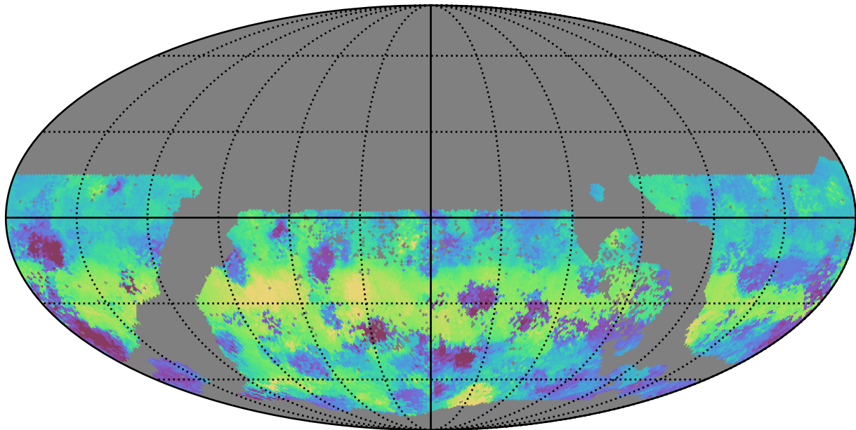
too_elab_heavy_r128_d3_gz_v3.4_10yrs WFD g band: Median HA
