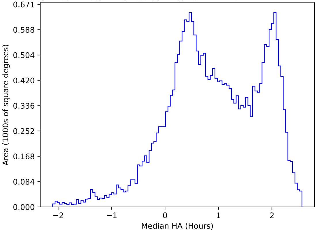
too_elab_heavy_r128_d3_gz_v3.4_10yrs All sky z band: Median HA
