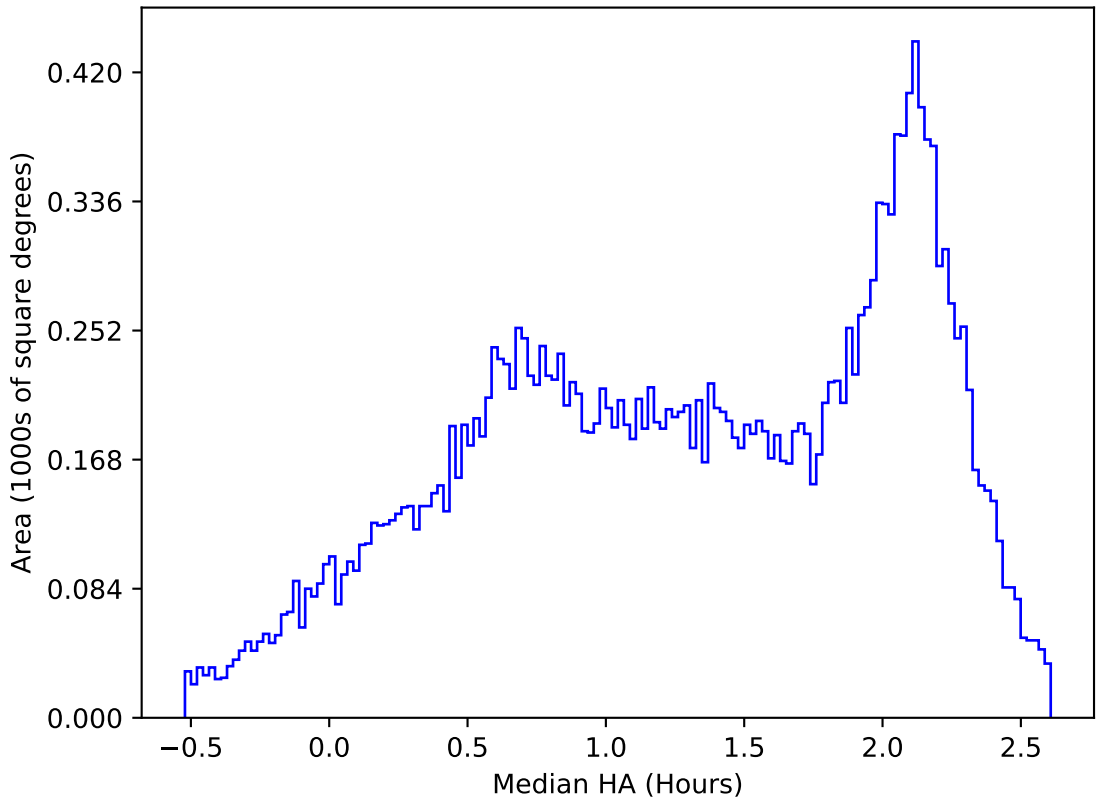
too_elab_heavy_r128_d3_gz_v3.4_10yrs All sky y band: Median HA
