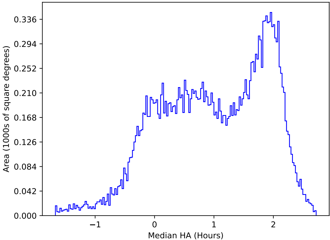
too_elab_heavy_r128_d3_gz_v3.4_10yrs All sky u band: Median HA
