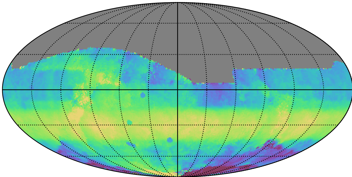
too_elab_heavy_r128_d3_gz_v3.4_10yrs All sky i band: Median HA
