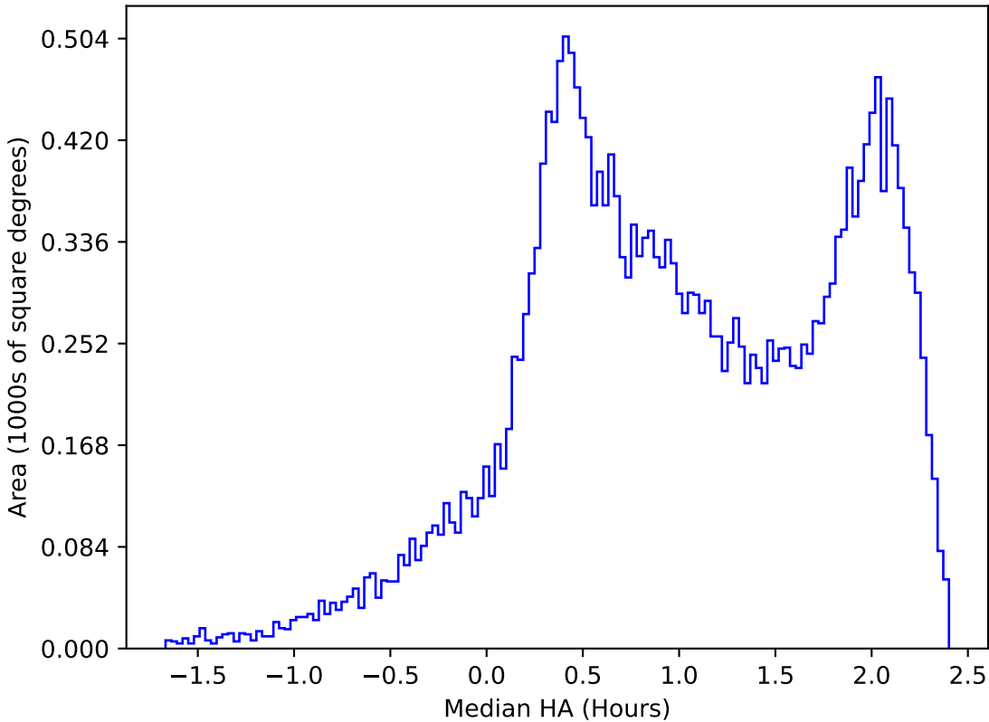
too_elab_heavy_r128_d3_gz_v3.4_10yrs All sky i band: Median HA
