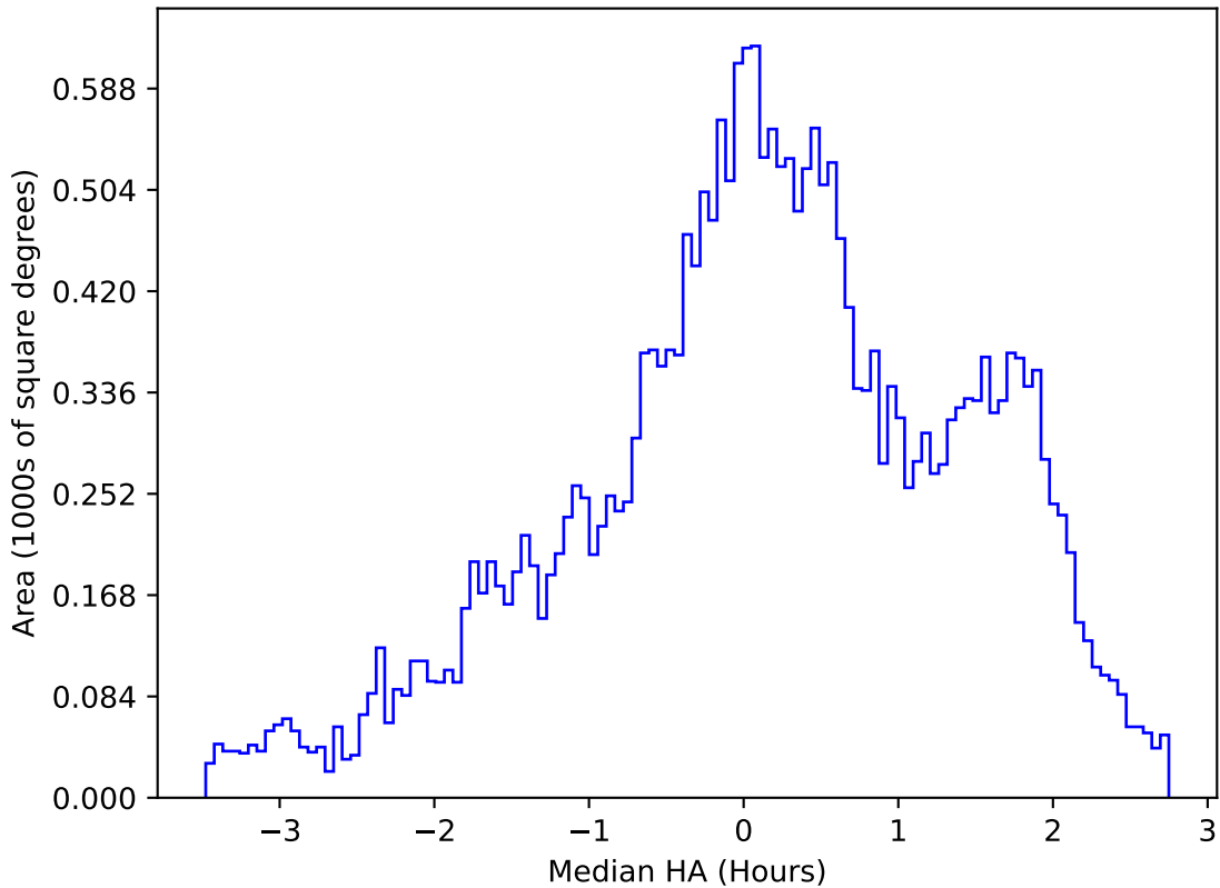
too_elab_heavy_r128_d3_gz_v3.4_10yrs All sky g band: Median HA
