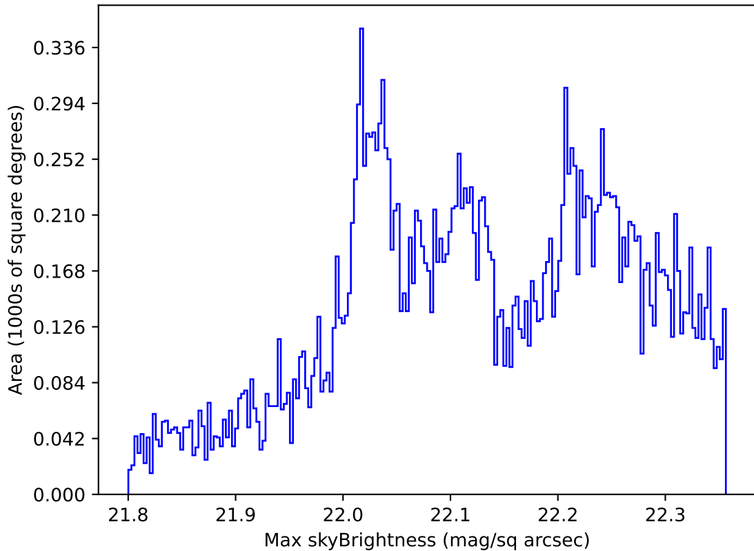
too_elab_heavy_r128_d3_gz_v3.4_10yrs All sky g band: Max skyBrightness
