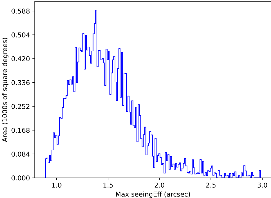
too_elab_heavy_r128_d3_gz_v3.4_10yrs Yr 1 z band: Max seeingEff
