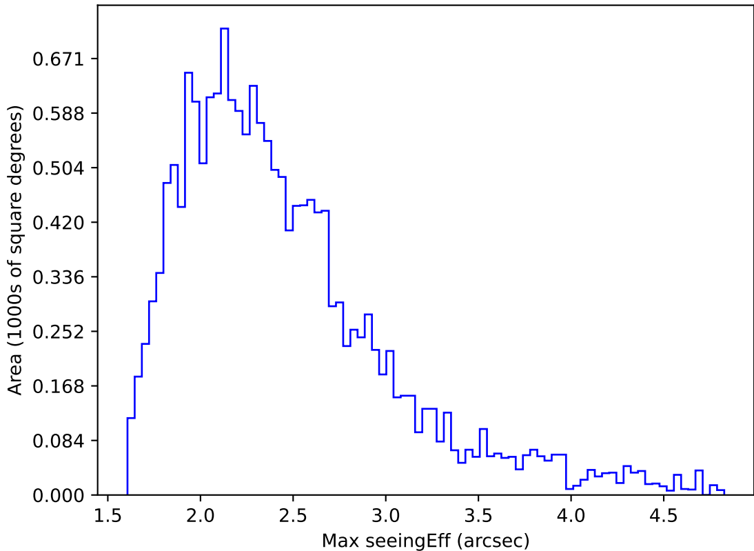
too_elab_heavy_r128_d3_gz_v3.4_10yrs WFD y band: Max seeingEff
