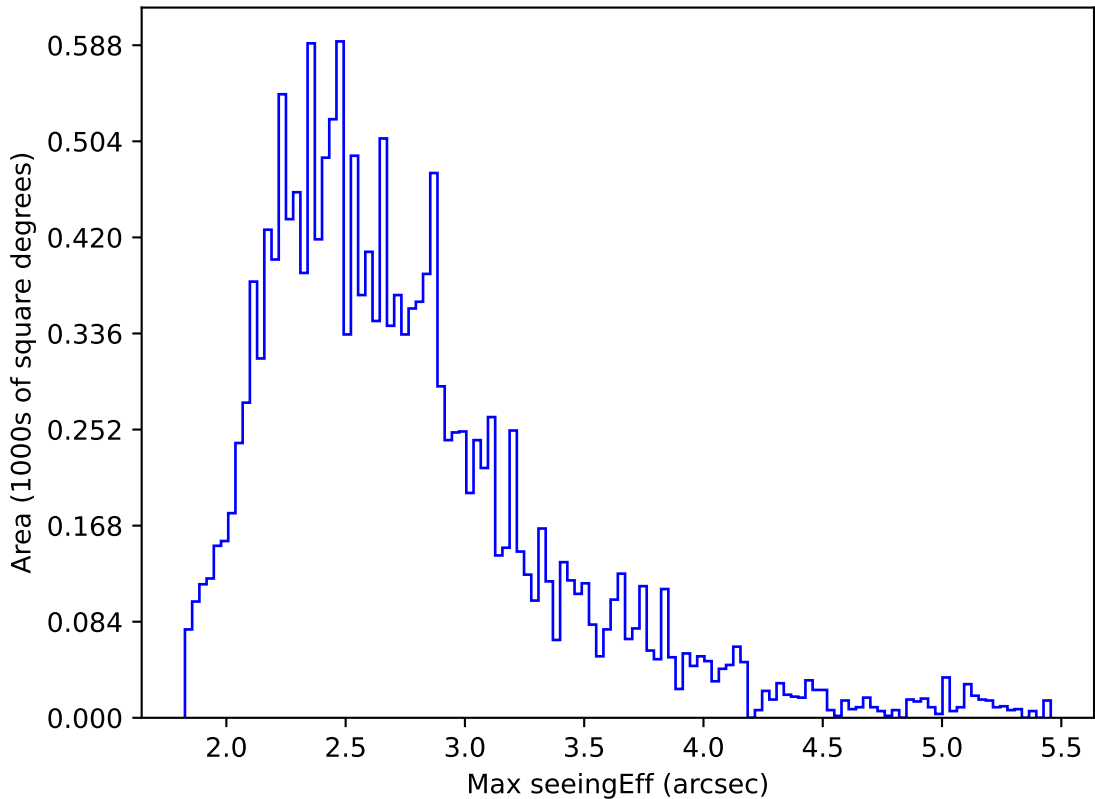
too_elab_heavy_r128_d3_gz_v3.4_10yrs WFD r band: Max seeingEff
