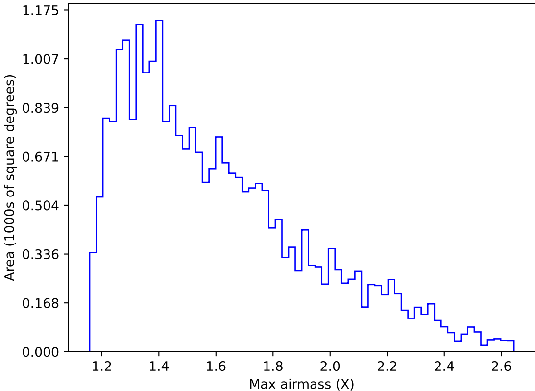
too_elab_heavy_r128_d3_gz_v3.4_10yrs Yr 1 z band: Max airmass
