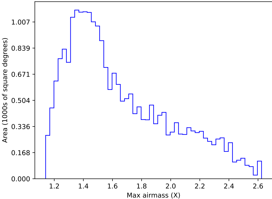
too_elab_heavy_r128_d3_gz_v3.4_10yrs Yr 1 y band: Max airmass
